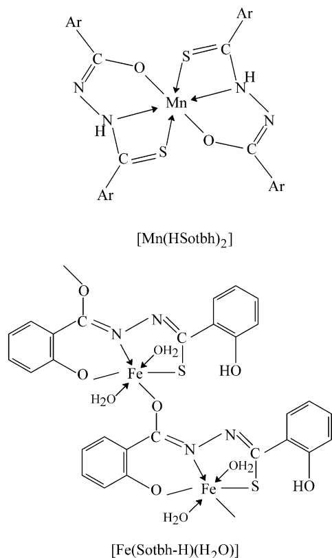
Figure 1. Proposed structure of the complexes of H 2 Sotbh.
