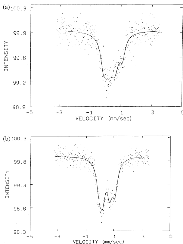
Figure 2. (a) Mössbauer spectrum of [Fe(Sotbh-H)(H 2 O) 2 ] at room temperature; (b) Mössbauer spectrum of [Fe(Sotbh-H)(H 2 O) 2 ] at 78\text{ K} .
